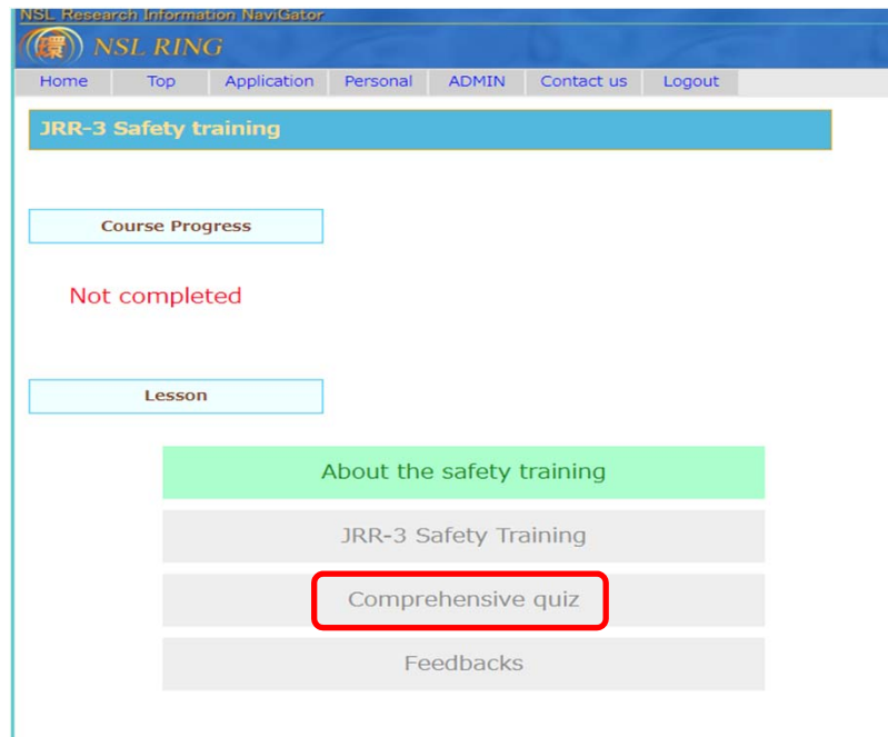
Fig.3 Comprehensive quiz
