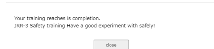
Fig6. Completion pop-up
