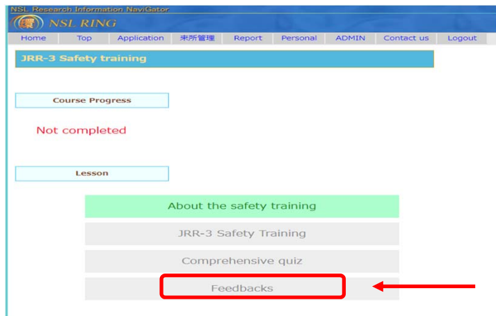
Fig. 5 Feedbacks
