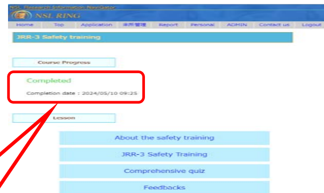
Fig.7b Completed
